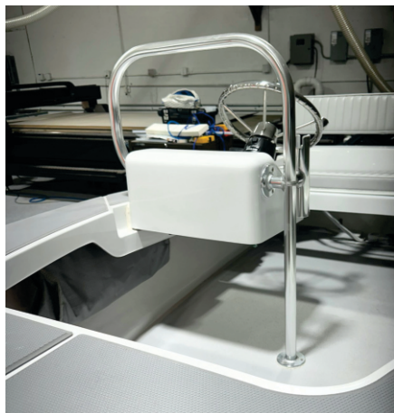
Side Console with aft bench seat
